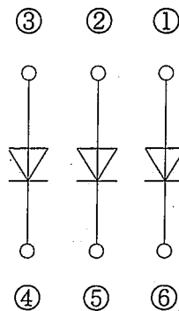
Equivalent circuit
